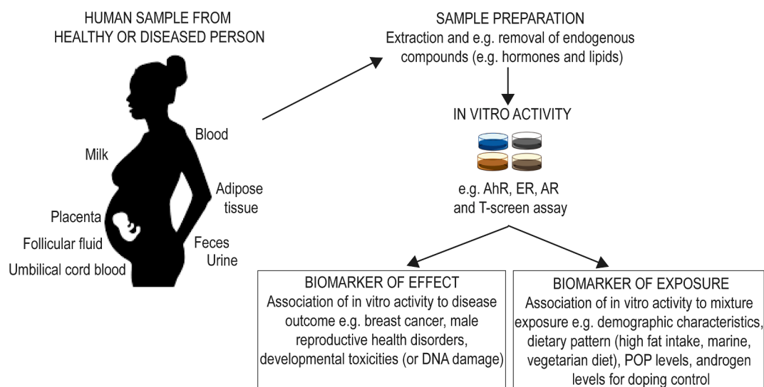
Fig. 3. Current alternative approaches for linking chemical exposures to health outcomes by using in vitro activities that take mixture effects of chemicals into account. Relevant human body fluids, tissues or secretions are selected from the cohort of interest and one or more in vitro assays analysing activation/inhibition of relevant key events for the disease in question are selected. The biological sample is typically undergoing an extraction and fractionation procedure that involves the extraction of a specific group of chemicals such as POPs or PFAS free from endogenous hormones. The measured in vitro activity can be used as a biomarker of effect by association with the disease outcome, or it can be used as a biomarker of exposure by association with demographic characteristics of the cohort population, their dietary profiles or exposure to specific chemicals.
