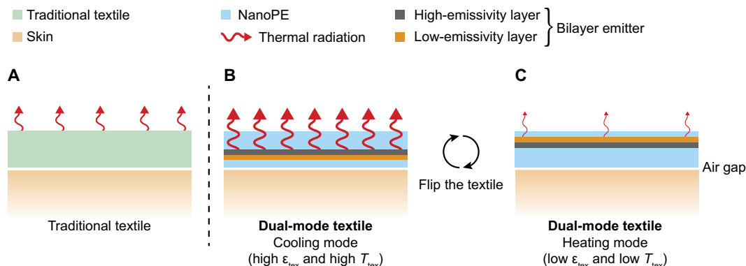
Fig. 1. Schematic of dual-mode textile. (A) Traditional textiles only have single emissivity, so the radiation heat transfer coefficient is fixed. (B) For a bilayer thermal emitter embedded in the IR-transparent nanoPE, when the high-emissivity layer faces outside and the nanoPE between the skin and the emitter is thin, the high emissivity and high emitter temperature results in large heat transfer coefficient, so the textile is in cooling mode. (C) The textile is flipped, and the low emissivity and low emitter temperature cause the heat transfer coefficient to decrease. The textile now works in heating mode.
